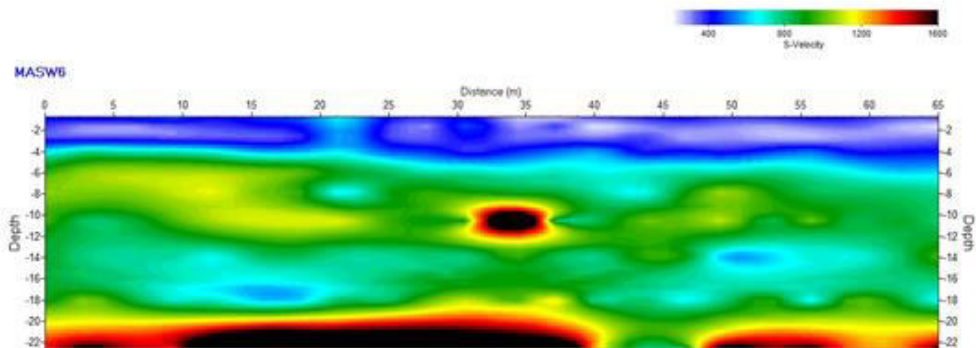
Figure 4- MASW6 2DVs model (22 source-receiver displacements, 3m interstation distance)
