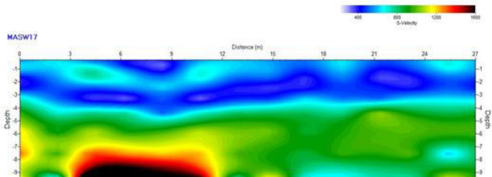
Figure 7-MASW17 2DV's model ((14 source-receiver displacements, 2 m interstation distance);
