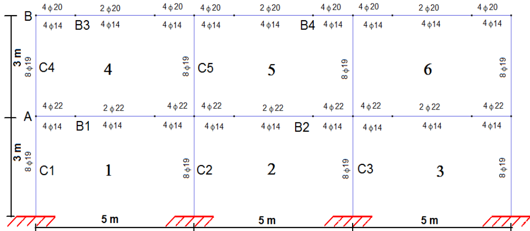
Figure 1- Frame geometry, support conditions, reinforcement, numeration of: beams, columns, joints and bays
