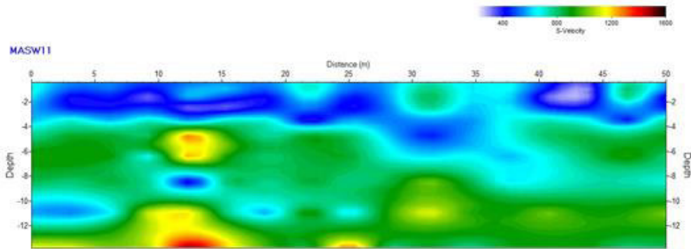
Figure 5-MASW11 2DV's model (17 source-receiver displacements, 3 meters interstation distance);
