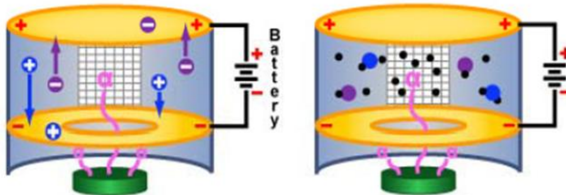
Ionization Smoke Alarm
